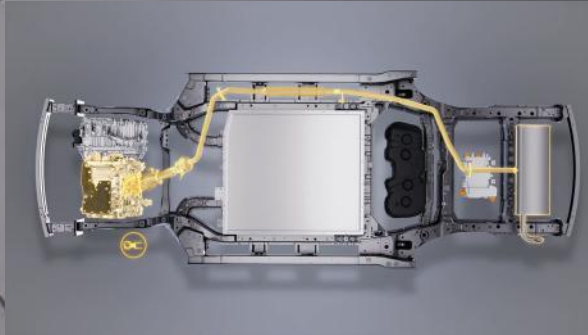
EXHAUST SYSTEM
