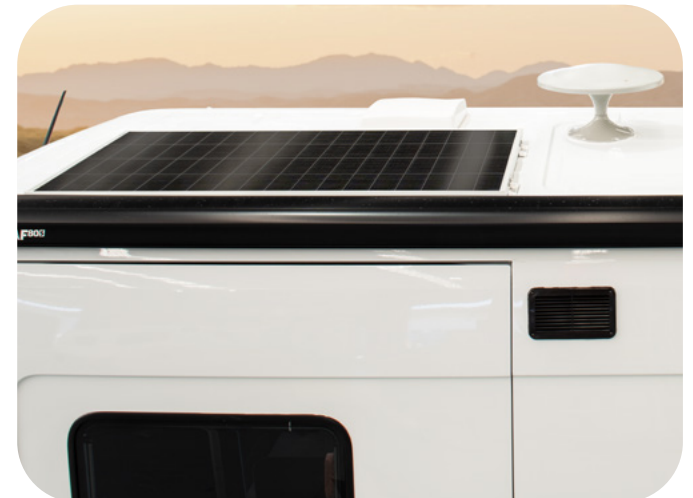
1x 200W solar panels powering 120AH Battery with twin-cell technology enhancing shaded performance
